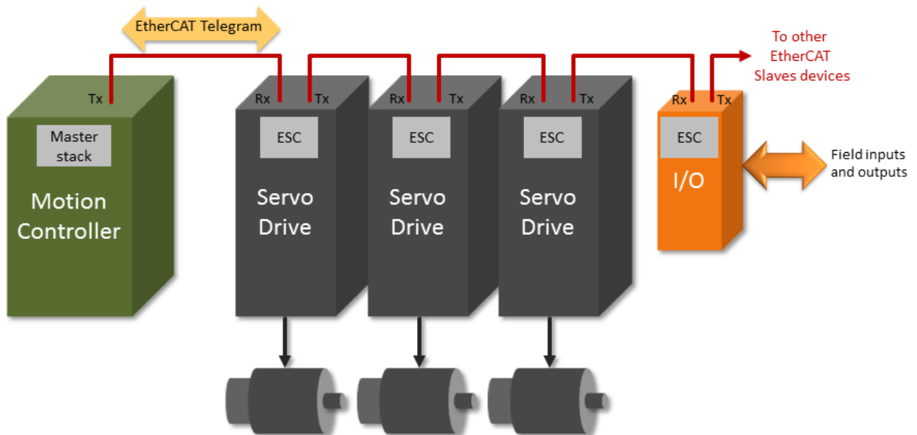
The most common EtherCAT configuration used in motion control is the "Line" connection
