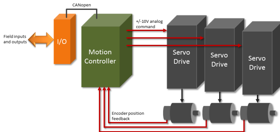
Traditional 3-axis analogue servo system requires at least 10 wires per axis.
